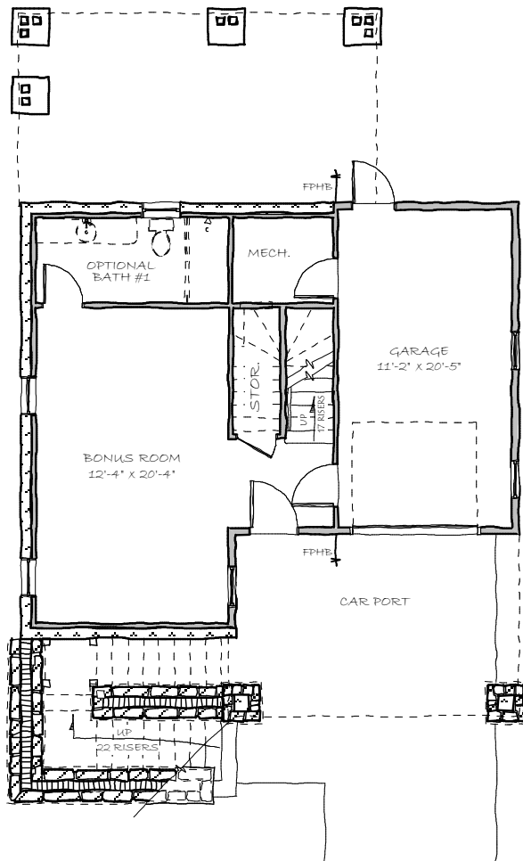
LOWER LEVEL FLOOR PLAN SCALE: 3/32" = 1'-0"
