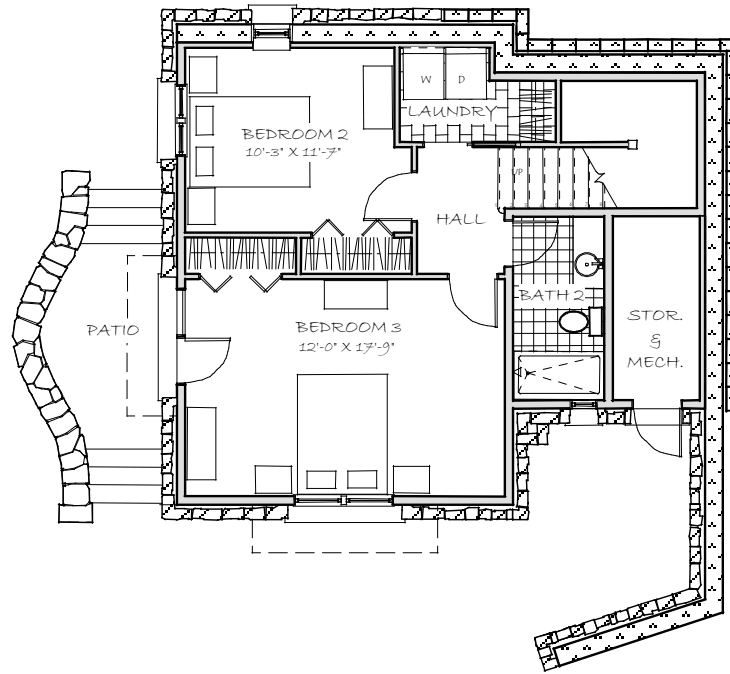
LOWER LEVEL FLOOR PLAN (UNIT 9)
